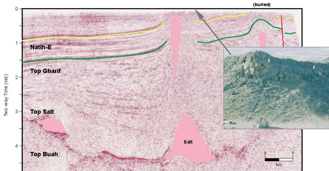
Figure 7: Oman, Ghaba salt basin, seismic section through Qarn Alam salt dome and surface indications (Peters et al., 2003)
