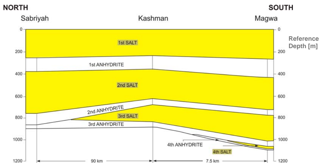
Figure 2: Stratigraphic cross section Gotnia Salt Formation (Ali, 1994)
