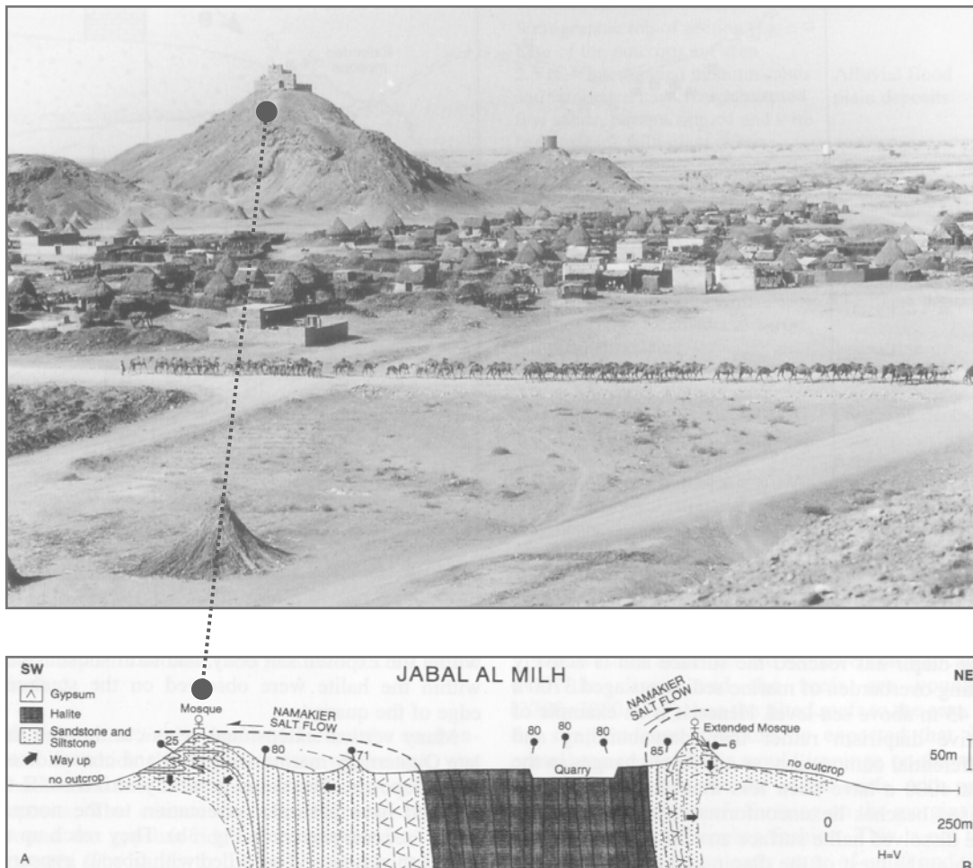
Figure 8: Outcropping Jabal Al Milh Salt Dome with residues, approx. 50 km north of well known Al Salif Diapir (Davison et al., 1996)
