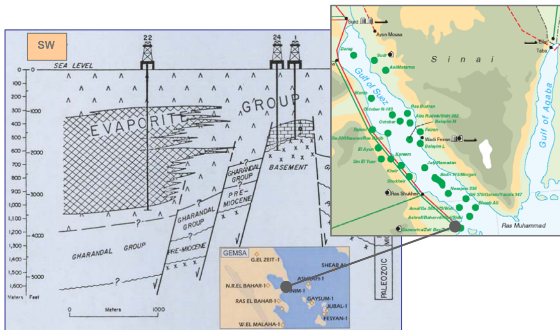
Figure 10: Gulf of Suez – gas & oil infrastructure (World Energy Atlas, 2002) and salt occurrence.
