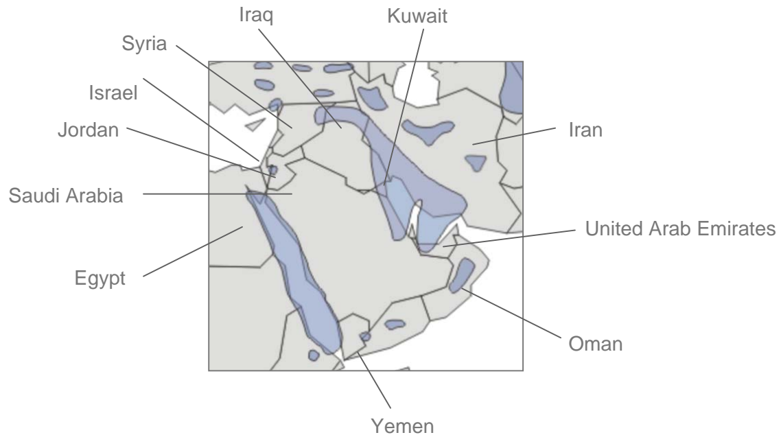
Figure 1: Map of Underground Salt Deposits in the Middle East (Folle, 2004)
